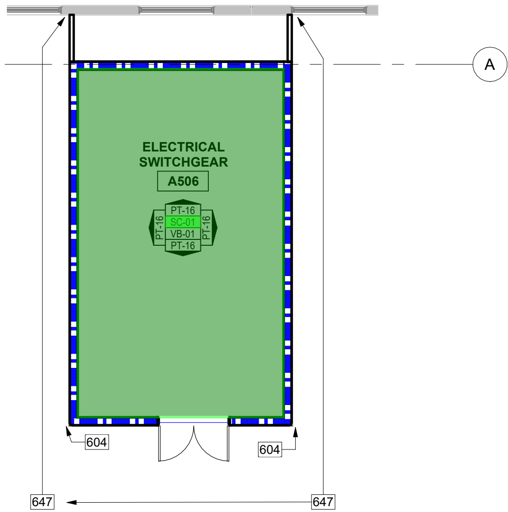
3 FINISH PLAN - ELECTRICAL SWITCHGEAR
