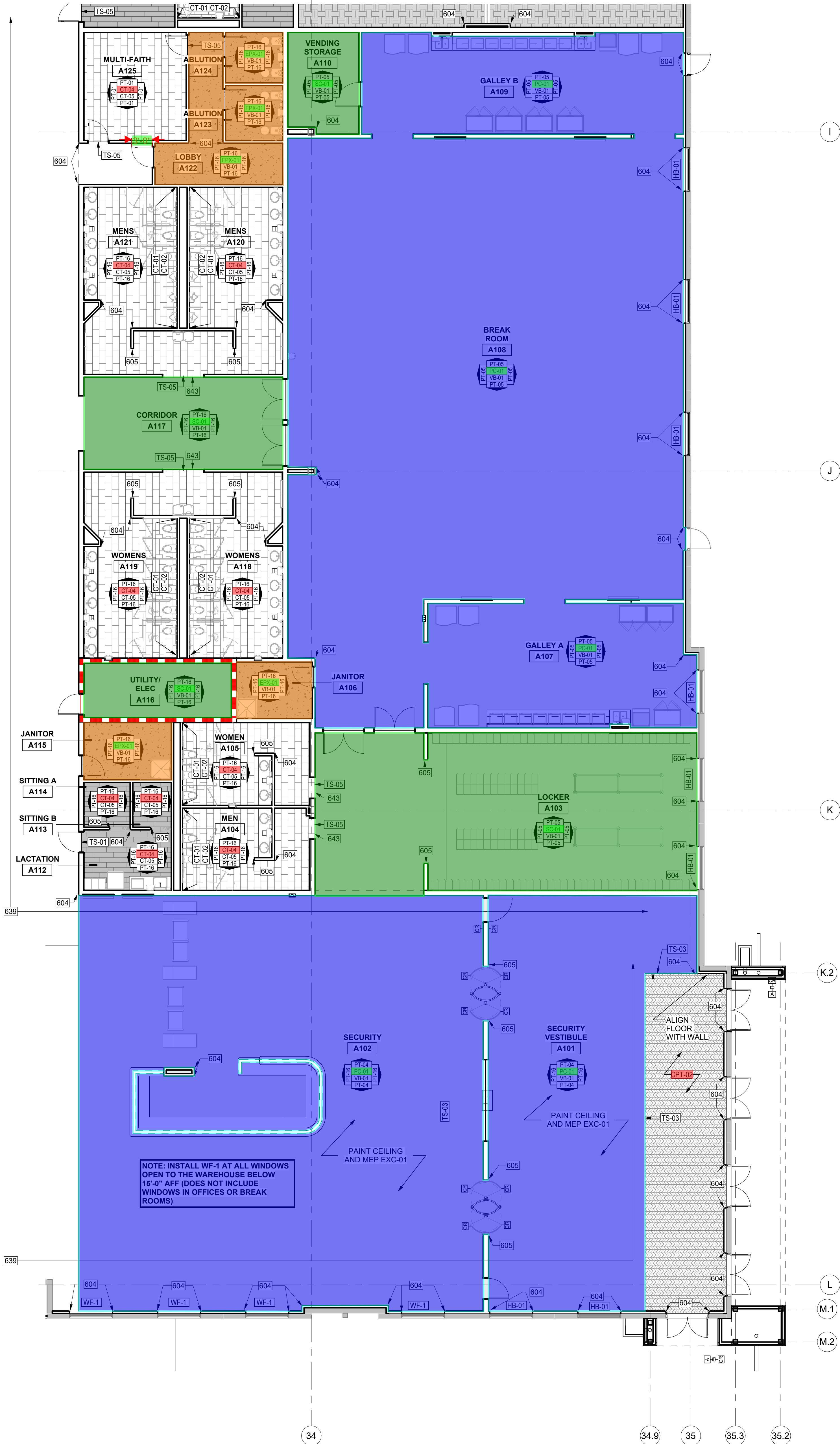
1 FINISH PLAN - MAIN OFFICE PLAN - 1
